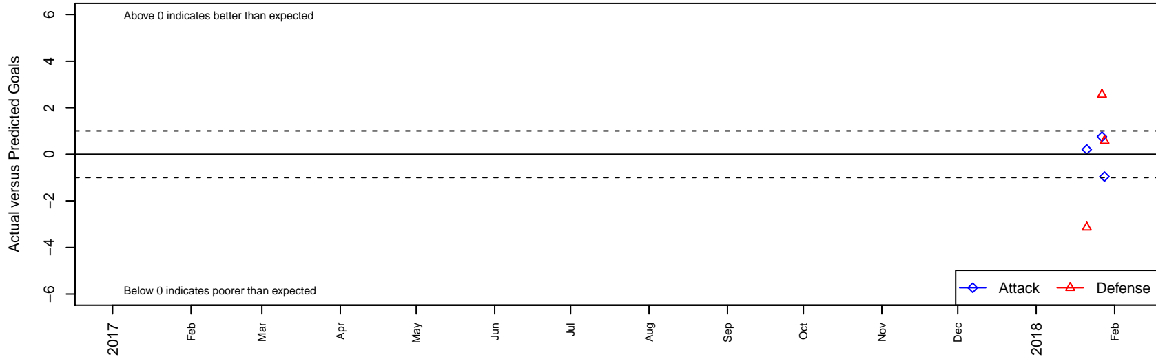
BSC Portland Black G02 Dots are actual minus expected GF (blue circles) and GA (red triangles). Blue line is smoothed change in attack strength. Red is smoothed change in defense strength.
